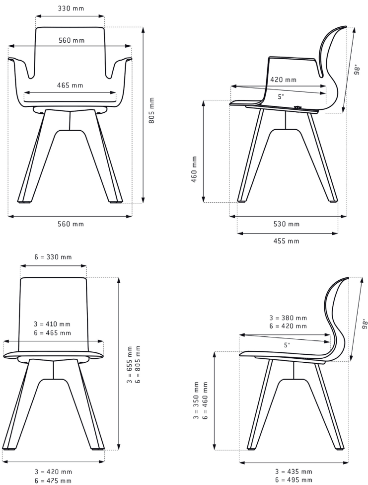
Dimensions for chair size 6
